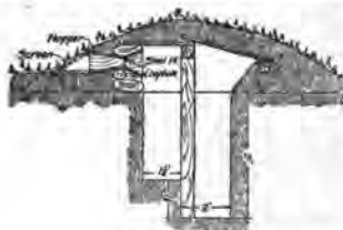
Enclosed Trench.
